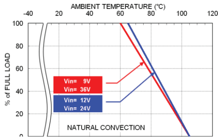
CWB15-24SXX Derating Curve
