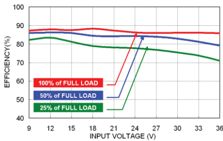
CWB15-24S5 Efficiency vs. Input Voltage
