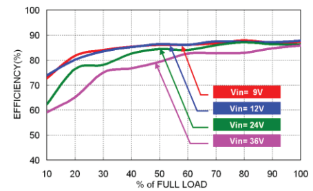
CWB15-24S5 Efficiency vs. Output Load
