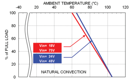
CWB15-48SXX Derating Curve
