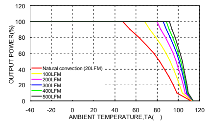
HWB150-48S05 Derating Curve (Note 3) With 0.45" Height Heat-sink
