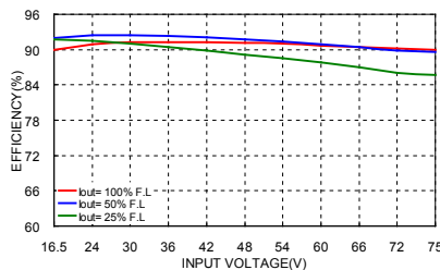
HWB150-48S05 Efficiency vs. Input Voltage
