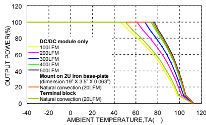
HWB150-48S05 Derating Curve (Note 3)
