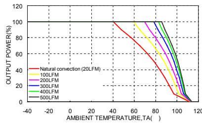
HWB150-48S05 Derating Curve (Note 3) With 0.24" Height Heat-sink
