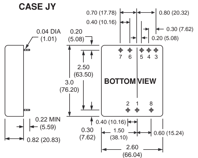
All Dimensions are in inches (mm)
