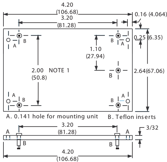
MODEL S-5 (For single and dual voltage units Cases A, A1, B, C, D) NOTE 1: For 2.2" AC pin spacing specify S-5/22
