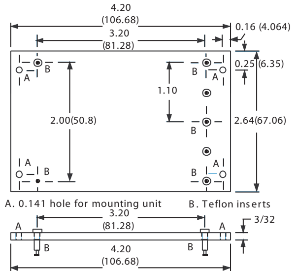
MODEL S-7 (For triple voltage units Cases C, D)
